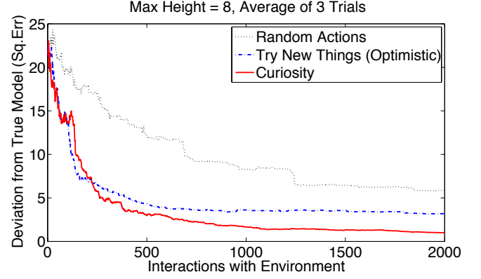
Fig. 5. Comparison of learning efficiency (deviation between current predictor weights and the optimal ones) in a simulated version of block-world (see text for details). The comparison is between a purely random policy, a policy for trying things not tried before — which acts randomly once all things have been tried — and our method of learning-progress-based artificial curiosity.
