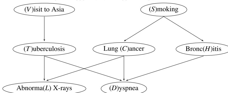
FIGURE 2. The 'Asia' Bayesian network.
