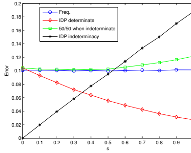
Figure 6. Error as a function of s for n_1 = n_2 = 20 , \gamma = 0.1 and \Delta = 0 . Here “Freq” denotes the MWW test.
