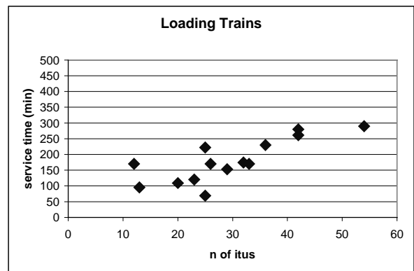
Figure 1. Time required to load a train vs. the number of ITUs to be moved.
