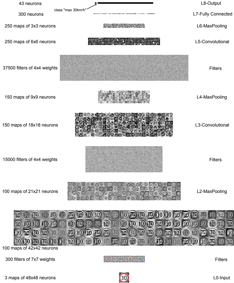
Figure 3: DNN architecture from Table 1 together with all the activations and the learned filters. Only a subset of all the maps and filters are shown, the output layer is not drawn to scale and weights of fully connected layers are not displayed. For better contrast, the filters are individually normalized.
