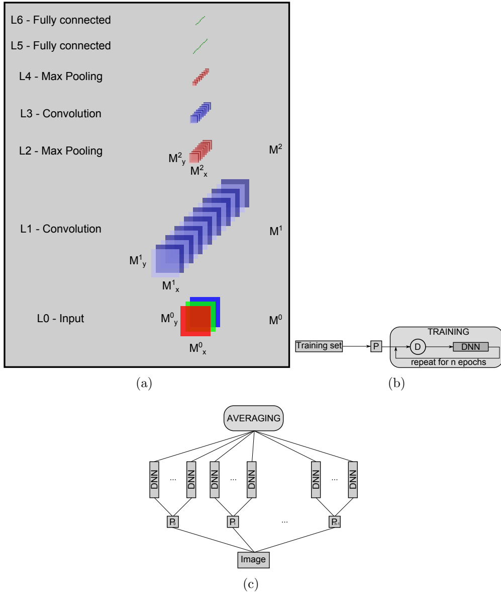
Figure 1: (a) DNN architecture. (b) Training a DNN: The dataset is preprocessed (P) before training starts; during training all original or preprocessed images are randomly distorted before each epoch (D). (c) MCDNN architecture: The input image is preprocessed by n different preprocessors P_0 - P_{n-1} and an arbitrary number of columns is trained on each preprocessed input. The final predictions are obtained by averaging individual predictions of each DNN.
