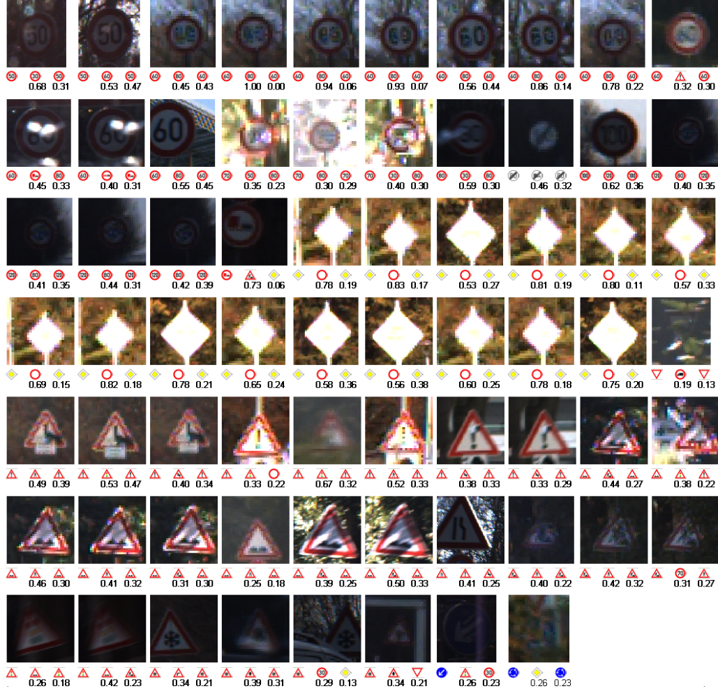
Figure 5: The 68 errors of the MCDNN, with correct label (left) and first (middle) and second best (right) predictions. Best seen in color.
