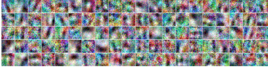
Figure 4: The learned filters of the first convolutional layer of a DNN. The layer has 100 maps each connected to the three color channels of the input image for a total of 3 \times 100 filters of size 15 \times 15 . Every displayed filter is the superposition of the 3 filters that are connected to the red, green and blue channel of the input image respectively. For better contrast, the filters are individually normalized.
