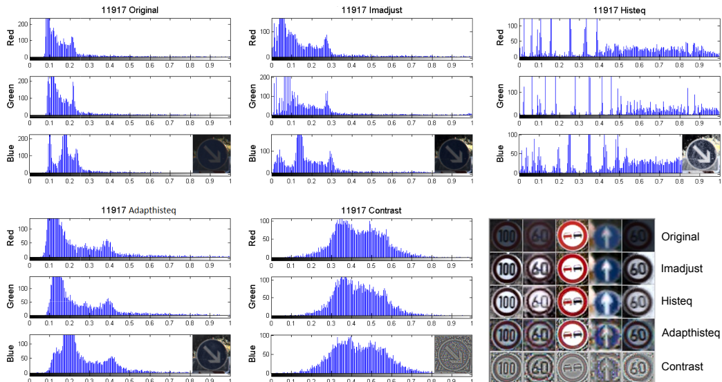
Figure 2: Histogram of pixel intensities for image 11917 from the test set of the preliminary phase of the competition, before and after normalization, as well as an additional selection of 5 traffic signs before and after normalization.
