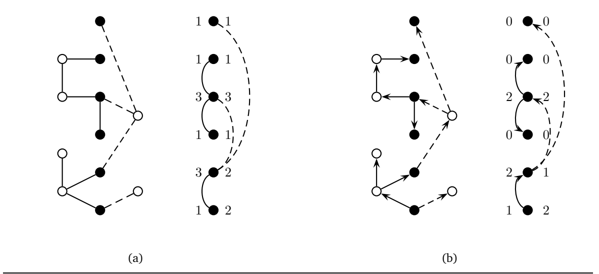
Figure 2 (a) Example of construction of (E_L, E_R, d_L, d_R) for DCST. On the left, the optimum solution OPT (dashed edges belong to OPT_R ). Black nodes belong to S . On the right, the edges E_L (full) and E_R (dashed). The degrees d_L and d_R are indicated at the left and right of each node, respectively. (b) Example of construction of (E_L, E_R, d_L^+, d_R^+) for DCOT, with an analogous notation.
