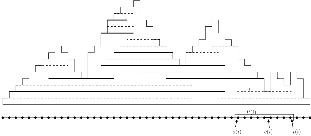
Figure 1: An example of capacity curve and the maze, with segments associated to some tasks T' (dashed) and m-tasks M' (bold). Note that (T', M') is 2-thin.
