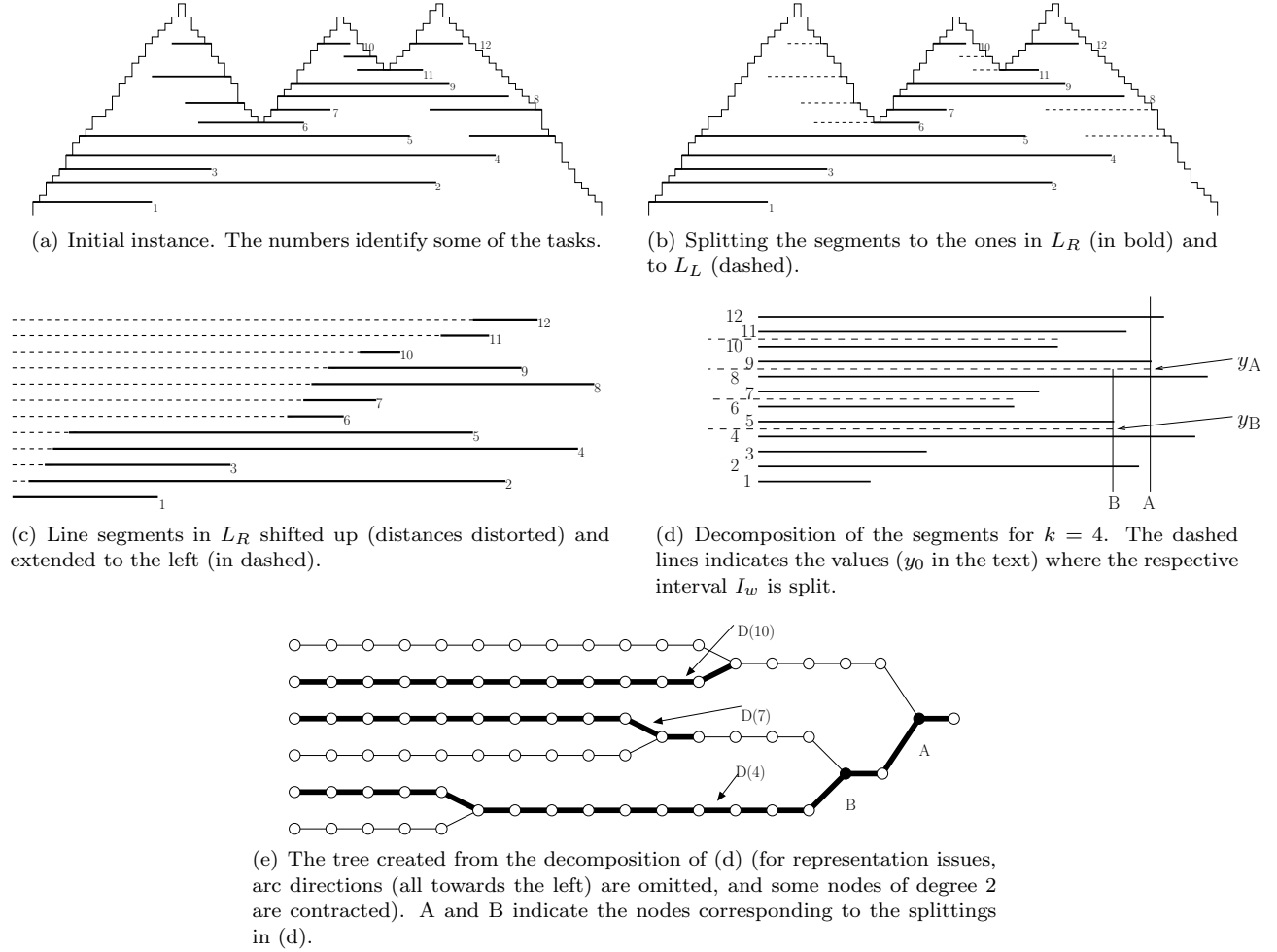
Figure 3: Construction of the maze
