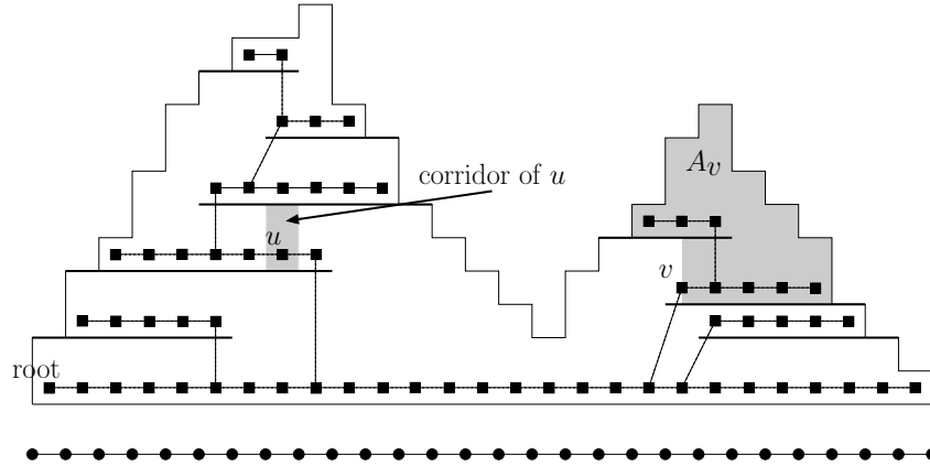
Figure 2: An example of a maze and the corresponding tree topology, in which tree nodes are represented by squares.
