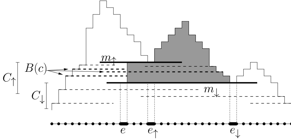
Figure 4: Tasks B \cup C_\downarrow \cup C_\uparrow (dashed) and area associated to a DP cell c . Tasks in C_\uparrow ( C_\downarrow ) use a common edge with m_\uparrow ( m_\downarrow ). Tasks (resp., m-tasks) that lie entirely within the shaded area are those that belong to T(c) (resp., M(c) ).
