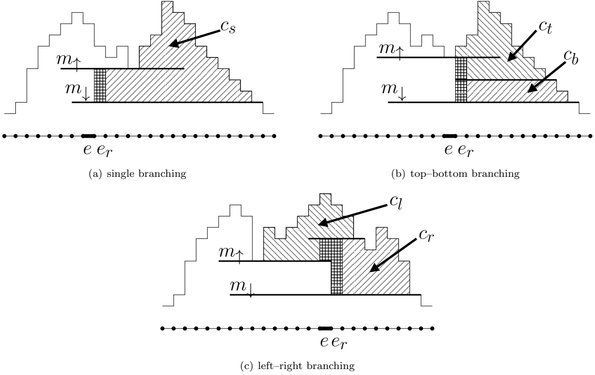
Figure 5: The three branching cases. The area of the cell c is the area of the subcell(s) c_s , (c_t, c_b) , and (c_l, c_r) , respectively, in addition to the checkered pattern.
