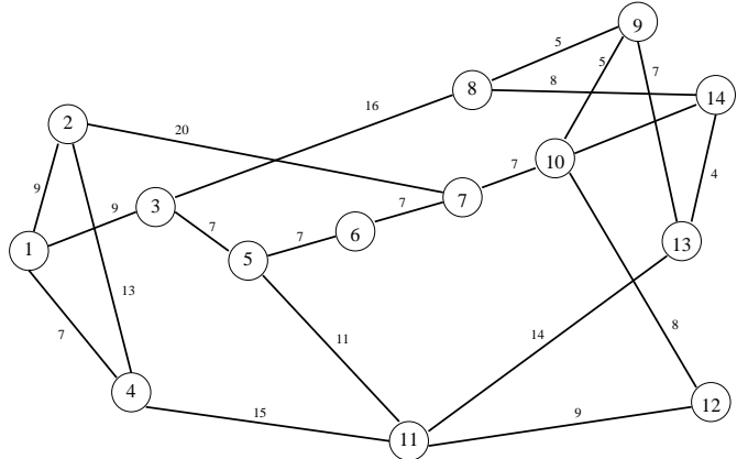
Figure 1: NSFNET. Numbers in circles are node identifiers. Each edge in the graph represents a pair of directed link and the numbers are propagation delays in msec.
